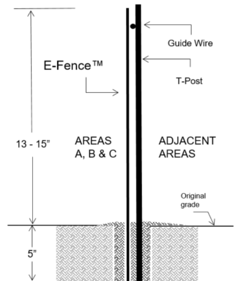
Fig. 2: Simple E-Fence configuration
