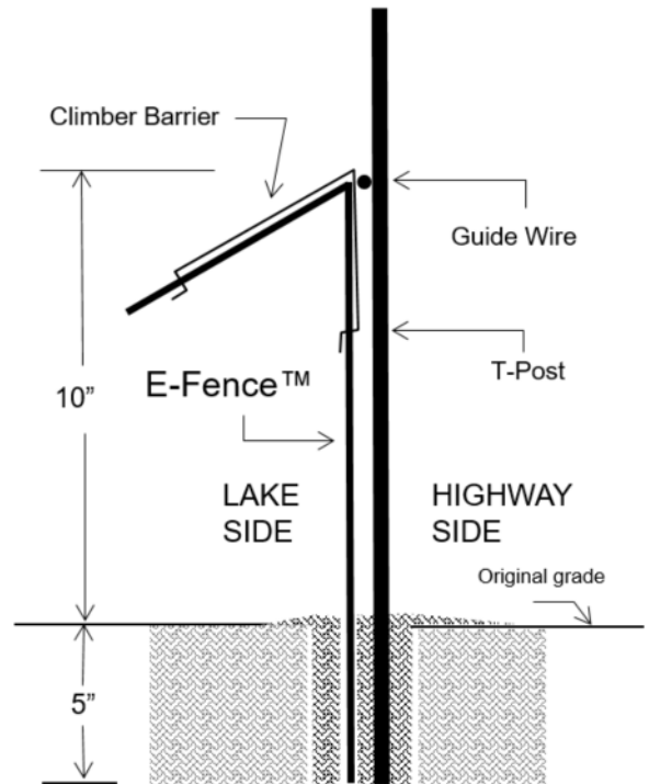
Fig 3: E-Fence™ with a climber barrier along HWY 1
